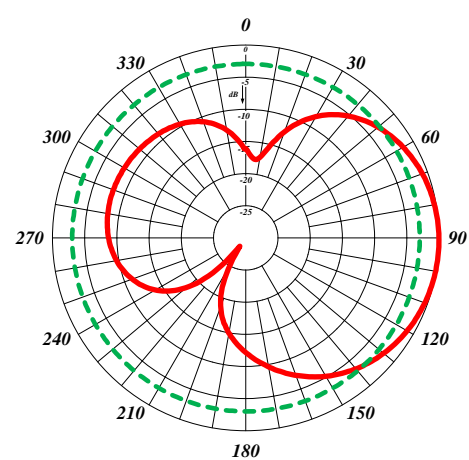
Vertical Pattern
