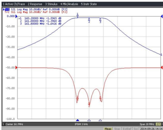
Antenna to 160-162 MHz Port
