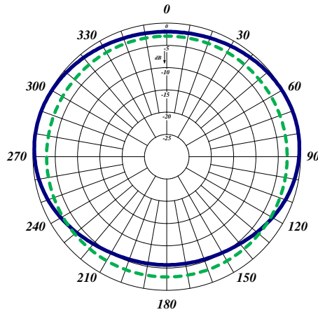
Horizontal Pattern (160MHz)
