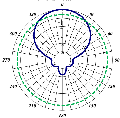
Horizontal Polarization
