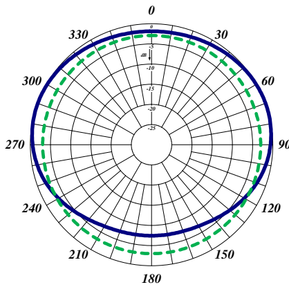
Horizontal Pattern (220MHz)
